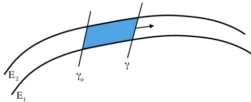
FIG. 2: A phase space region moves from one cell to next in the time \tau_0 \sim \hbar/\Delta E .
