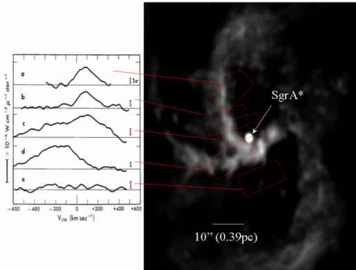
Figure: First evidence came from orbiting gas. Gas has radial velocities up to a few hundred km/s. Suggested a central mass of a few times 10^6 M_{\odot} .
